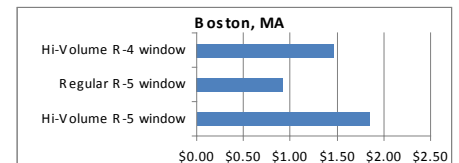
Present Value of Energy Savings per Dollar of Marginal Cost Compared to Typical ENERGY STAR® Windows
